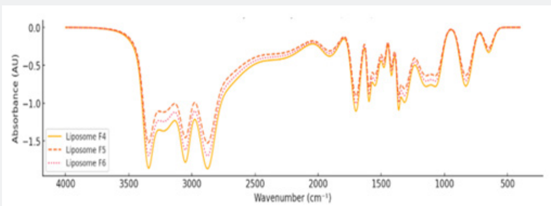
Figure 7: FTIR Graphs for F4-F6 Batch
