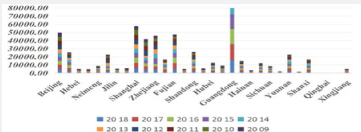
Figure 3: Data distribution of influencing factors in each city.
