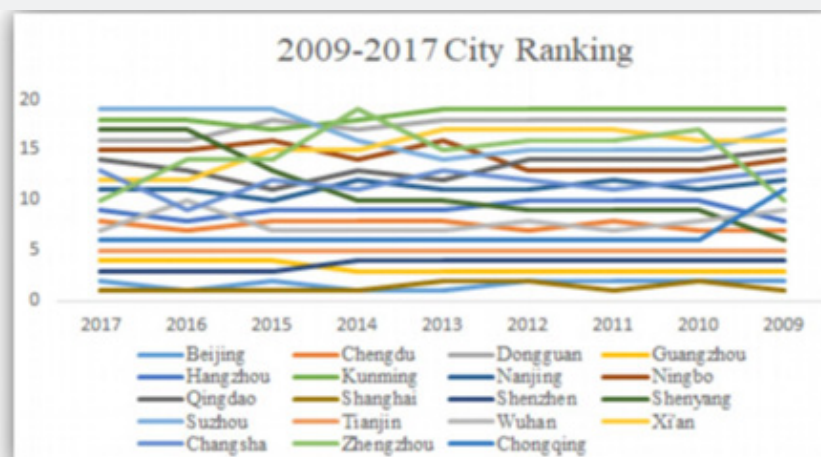
Figure 15: Regional rankings over the past decade.
