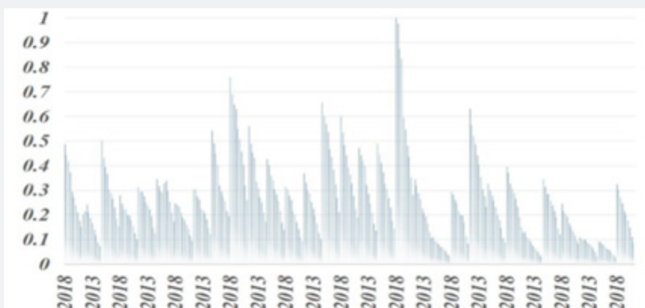
Figure 4: Standardized data distribution.
