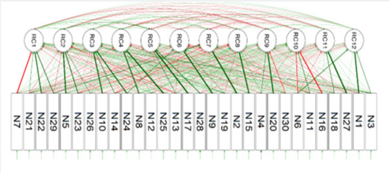
Figure 2: Path diagram.
