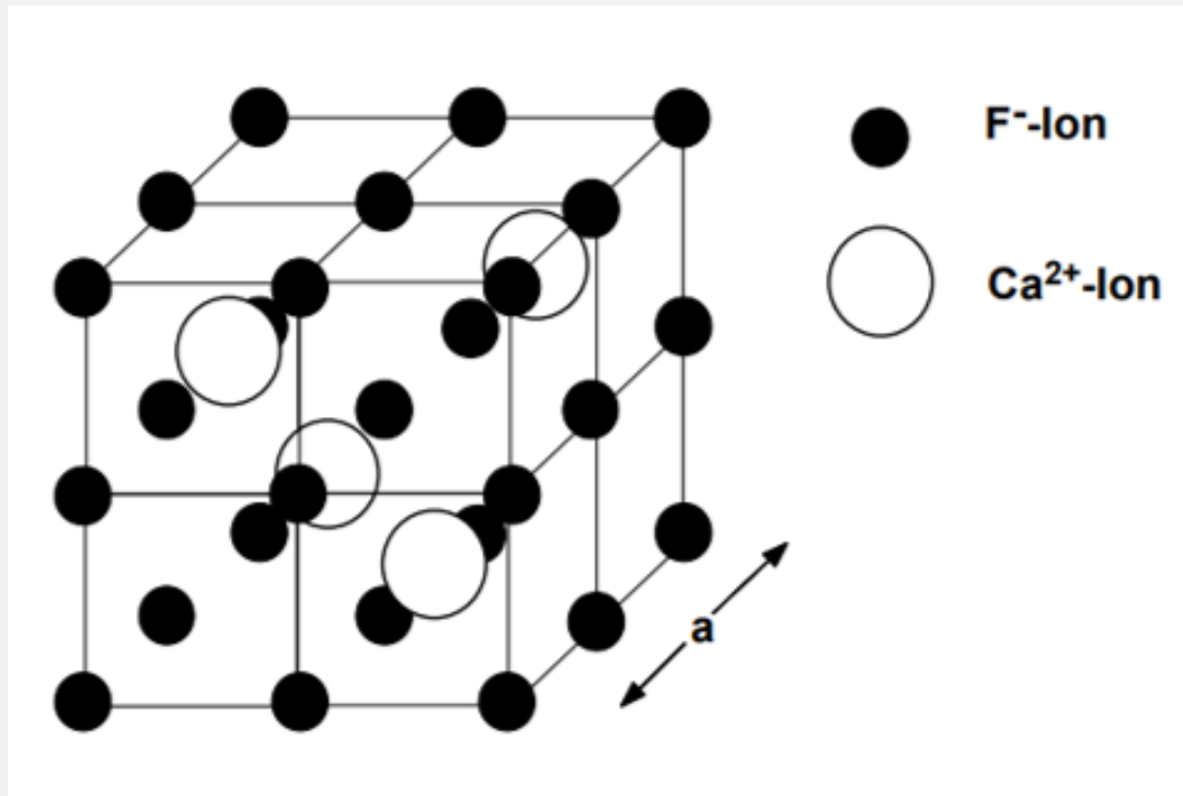
Figure 5: The crystalline structure of pure Calcium fluoride.
