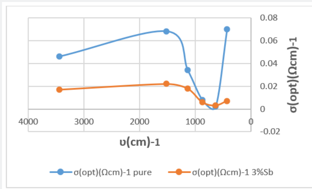
Figure 3: Shows the studying of the conductivity variations by the frequency function of pure calcium fluoride and the antimony doped calcium fluoride by (3wt%).
