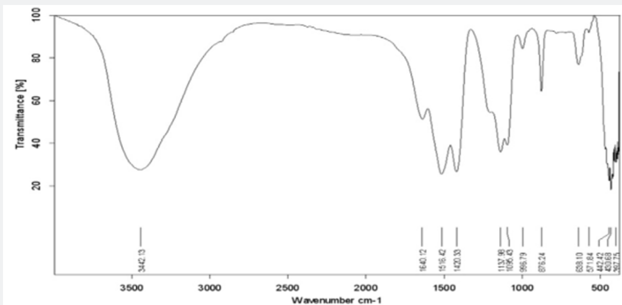
Figure 6: Shows the FTIR spectrum of Sb doped \text{CaF}_2 samples (3wt%).
