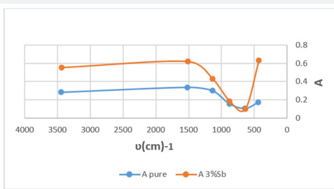
Figure 4: Absorbance variations by the frequency function of pure calcium fluoride powder and the antimony doped calcium fluoride by (3wt%).
