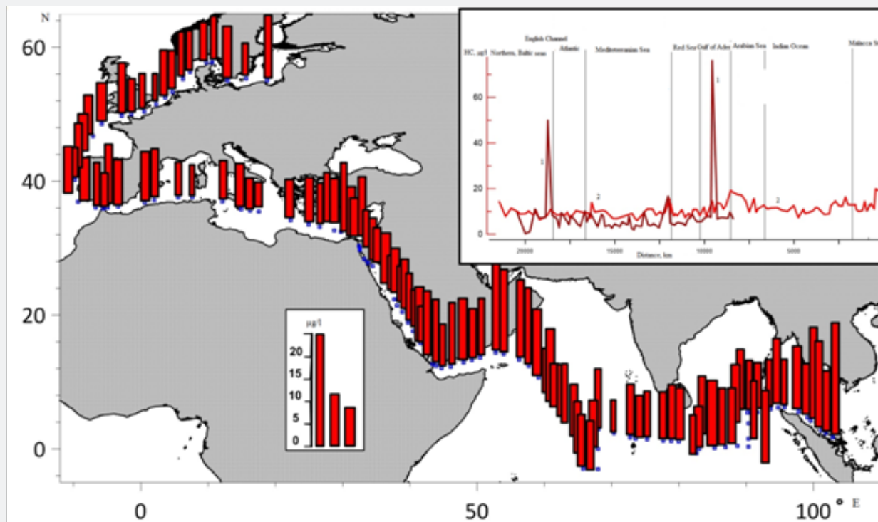
Figure 2: Distribution of hydrocarbons in surface waters in the cruise of R/V “Academician Boris Petrov” (columns). The inset: the distribution of hydrocarbons ( \mu g/l) in surface waters in cruises 1 -R/V “Akademik Nikolai Strakhov”, 2 - R/V “Akademik Boris Petrov”.
