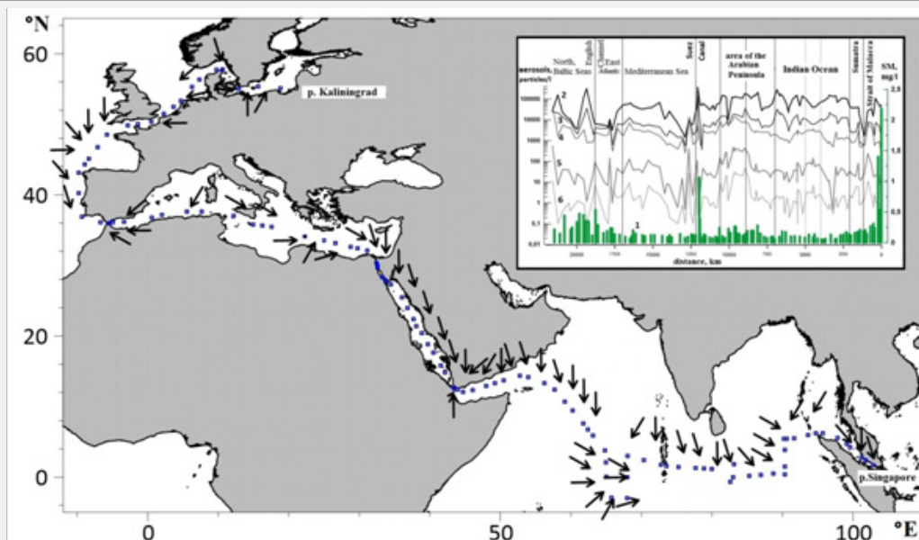
Figure 1: Sampling stations and the main wind direction along the route R/V “Academician Boris Petrov”. The inset: 1 - the distribution of suspended matter (columns, mg/l) and the granulometric composition of the aerosols ( \mu ) in the driving layer of the atmosphere: 2 - 0.3-0.5, 3-0.5-1, 4 – 1-3, 5 – 3-5, 6> 5.
