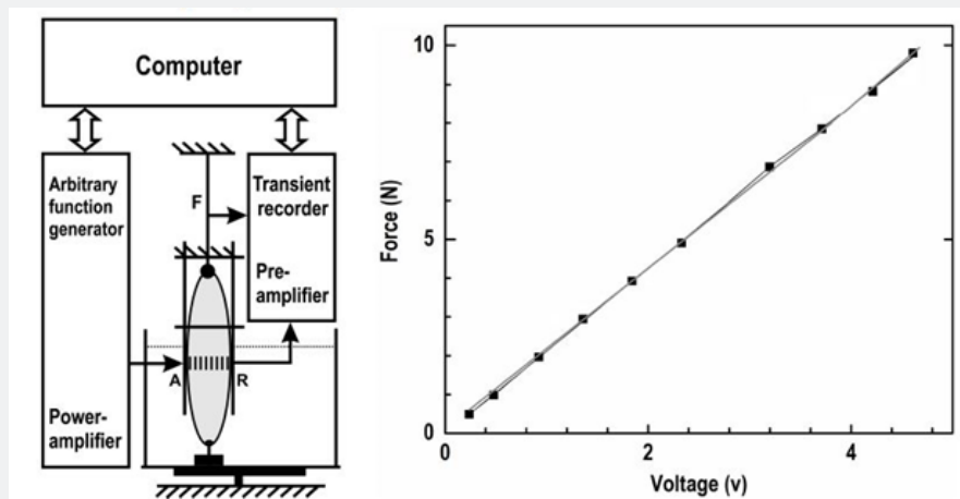
Figure 1: Block diagram (left) demonstrating the data acquisition set-up to record the TOF of ultrasonic waves traveling across the rat medial GM muscle for fixed (constant) distance between the transducers. The monitored muscle was surrounded with warmed paraffin oil and fixated in lateral dimensions by a custom-designed solid structure stabilized by an outer frame (stainless steel). Where A: Actuator, R: Receiver. The force sensor end is tightened with the string to the Achilles tendon of the medial GM muscle. Graph right representing the calibration data of the force sensors used for this monitoring. A linear fit has been used to determine the slope i.e. rate of change of force.
