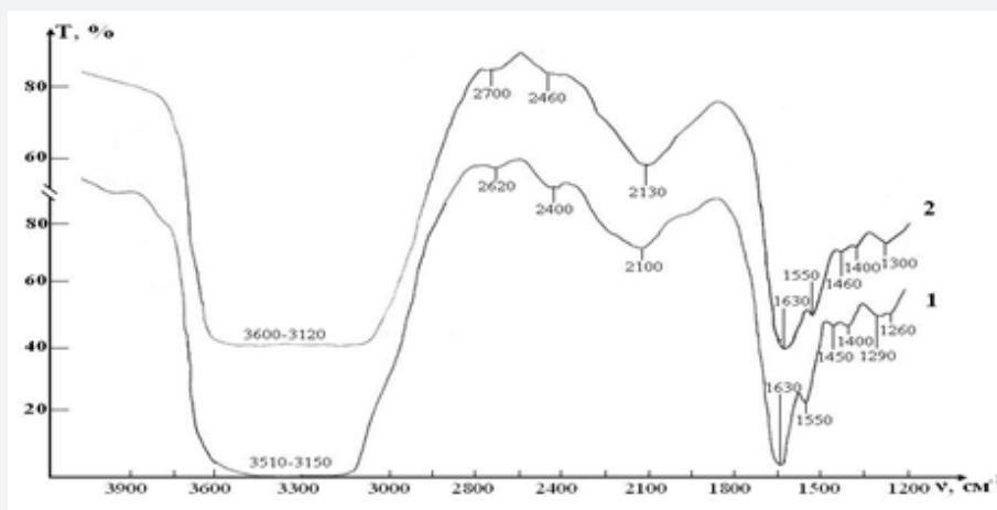
Figure 5: IR absorption spectra of initial erythrocyte suspensions in the range 1200-4000 \text{cm}^{-1} : curve 1- control; curve 2 - test.
