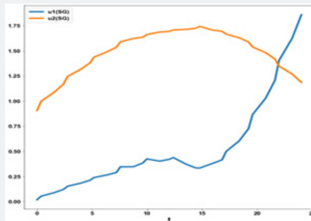
Figure 7: MNLMPc (u1 u2 with savitzky Golay filter).
