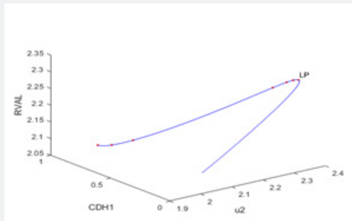
Figure 4: Bifurcation (full model u2 CDH1 Rval).
